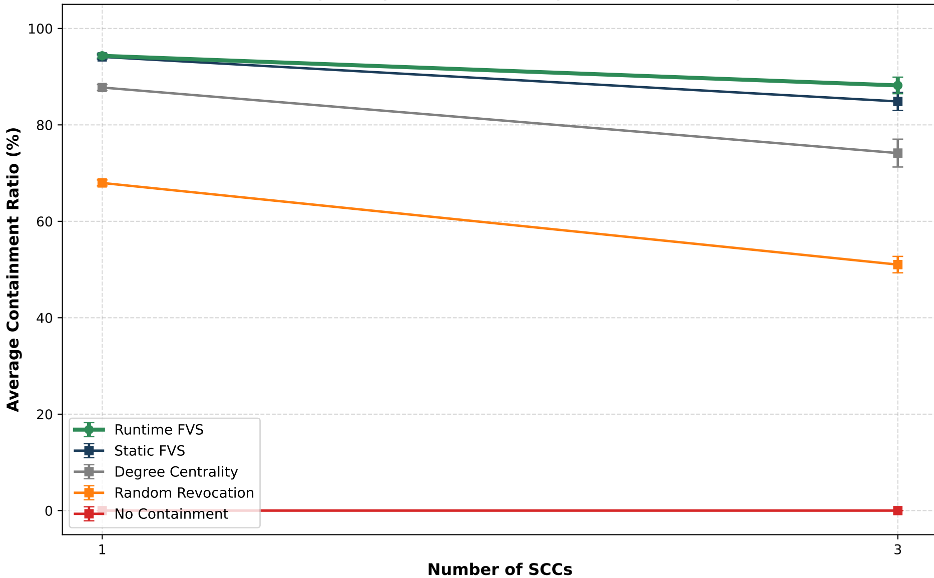
Efficacy Decay under Increasing Graph Complexity
